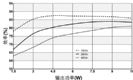
5: WK392812D-10 效率曲线
