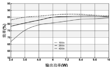
5: WK392812D-10 效率曲线
